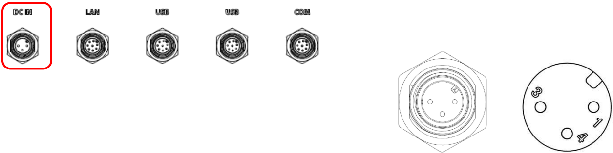
M12 DC-in(3-pin) Front View Pin Assignments
